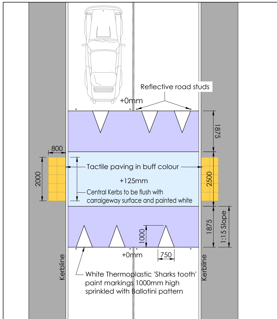
Detail 'C' - Speed Ramp
