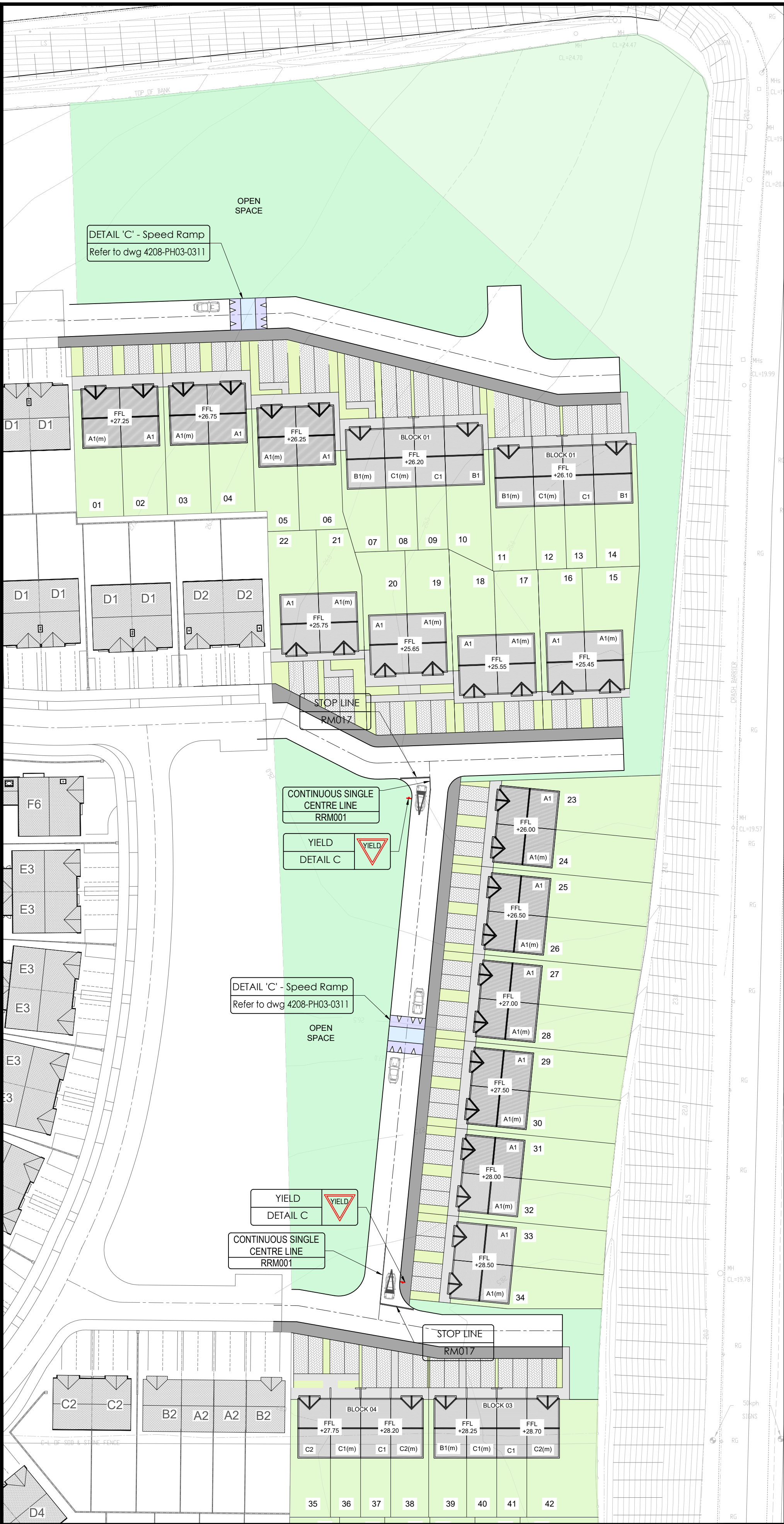
Site Layout (Northern Section) Scale 1:500
