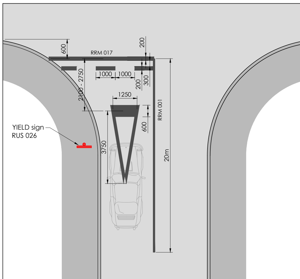
Detail 'B' - Typical YIELD Junction
