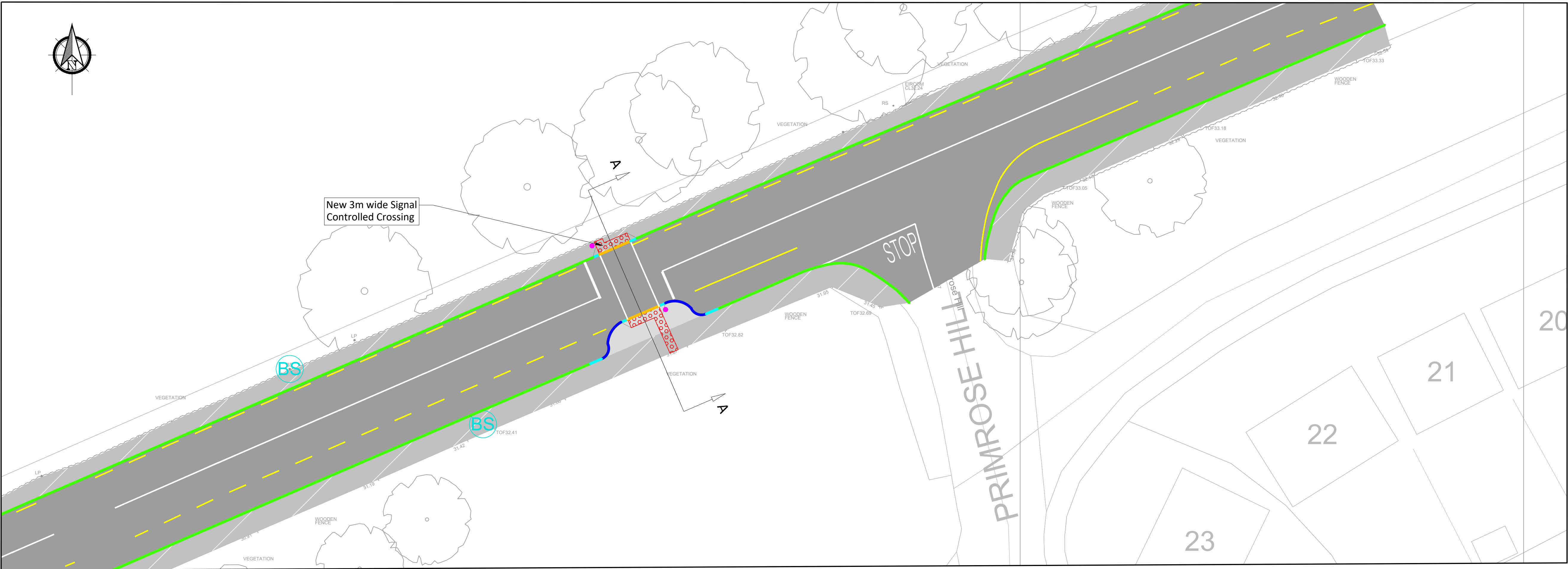
LOCATION PLAN SCALE 1:200
