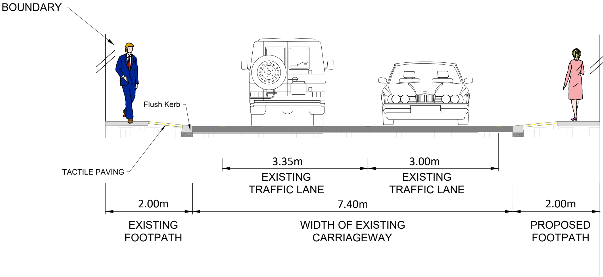
CROSS SECTION A-A SCALE 1:50
