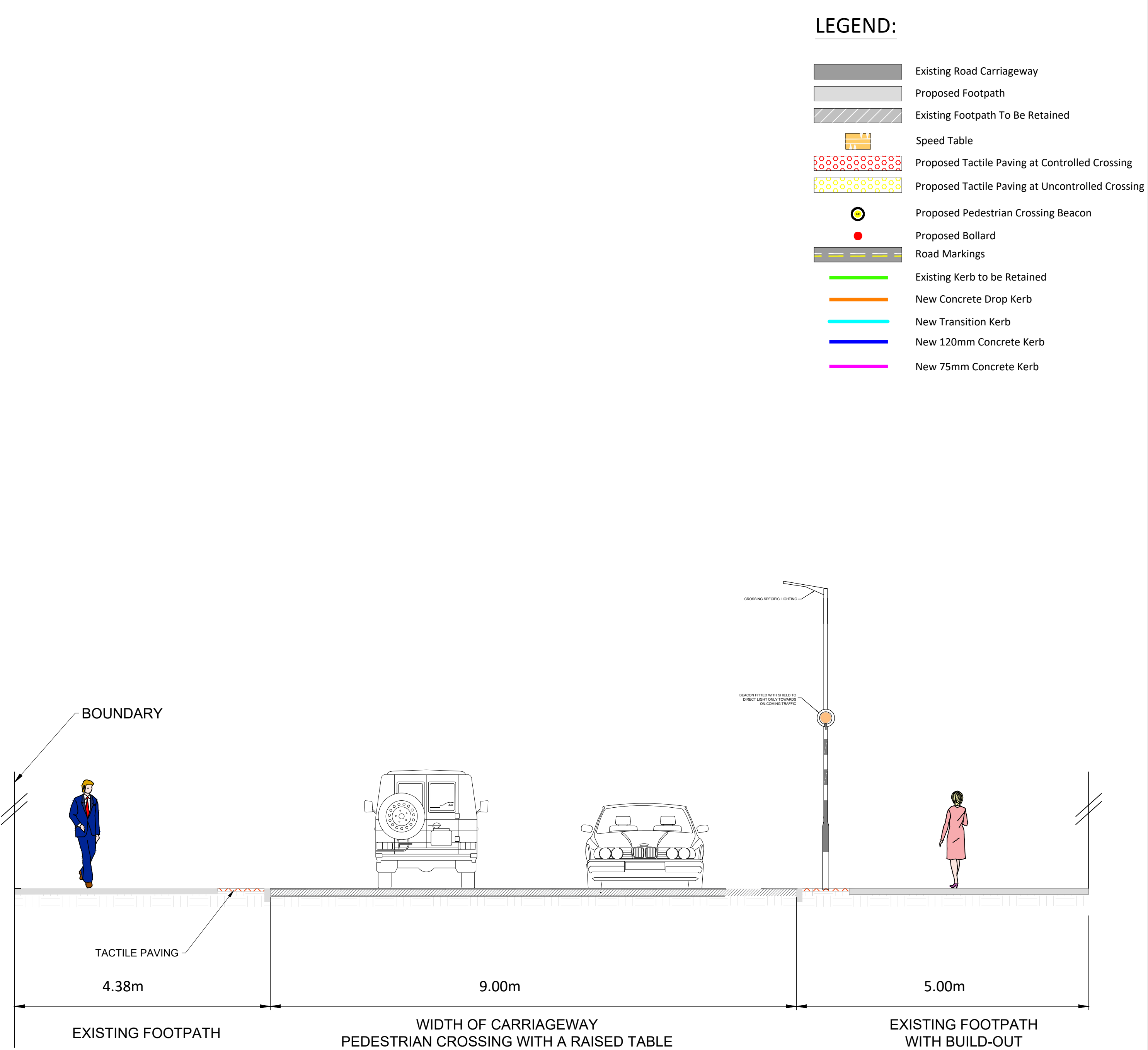
CROSS SECTION A-A SCALE 1:50
