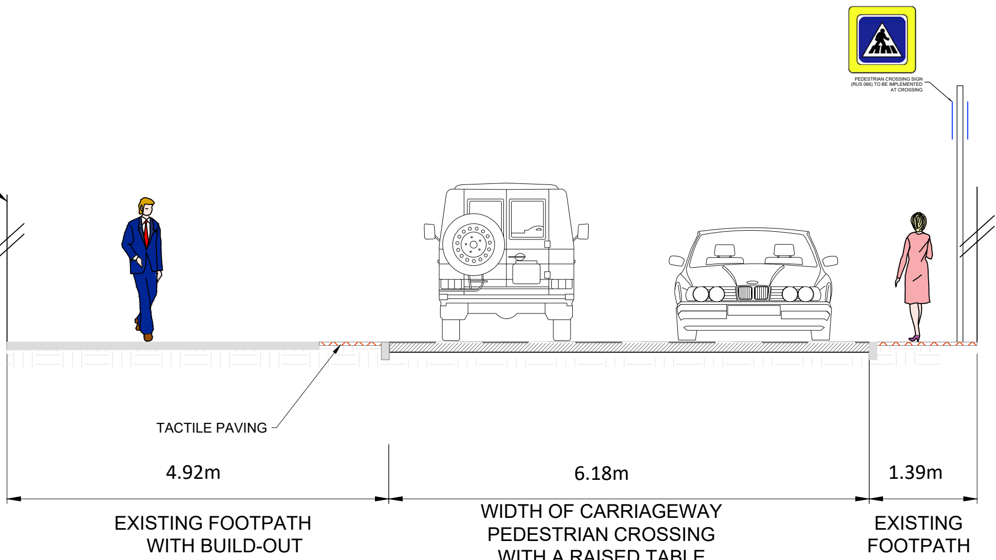
CROSS SECTION A-A SCALE 1:50
