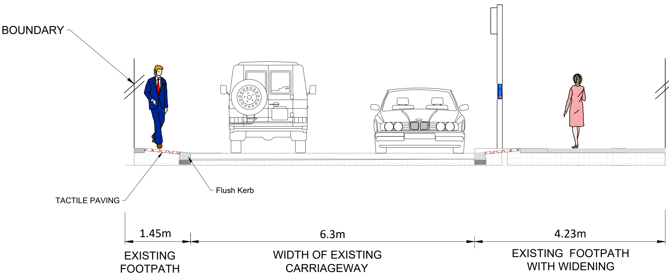
CROSS SECTION A-A SCALE 1:50
