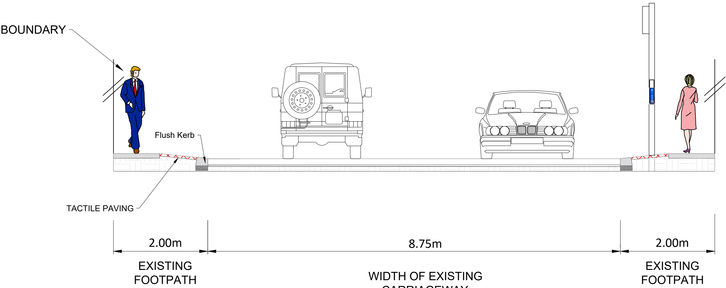
CROSS SECTION A-A SCALE 1:50
