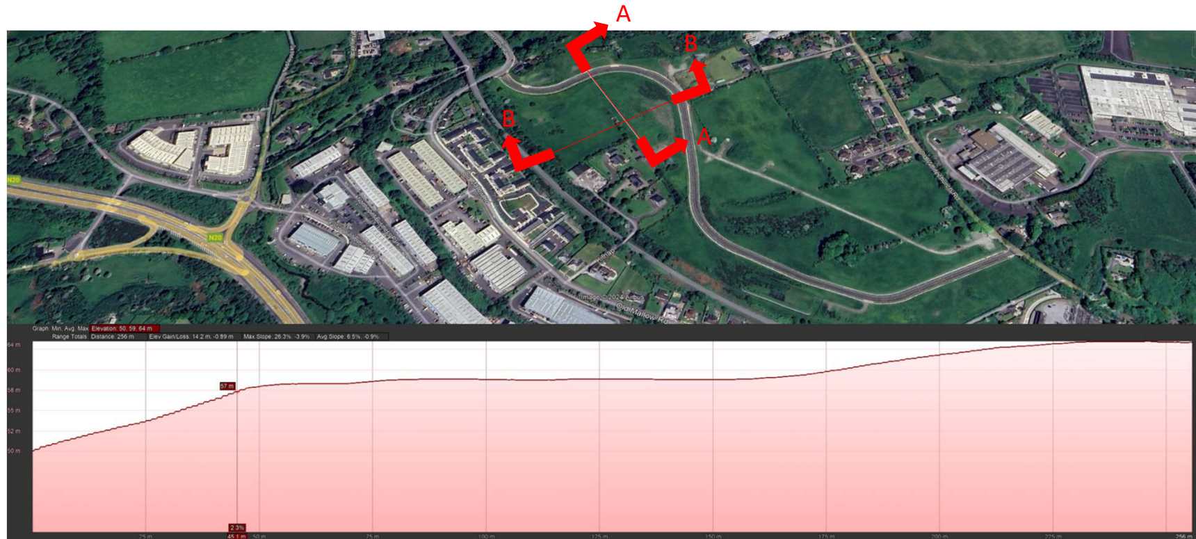
A-A North-South Section
