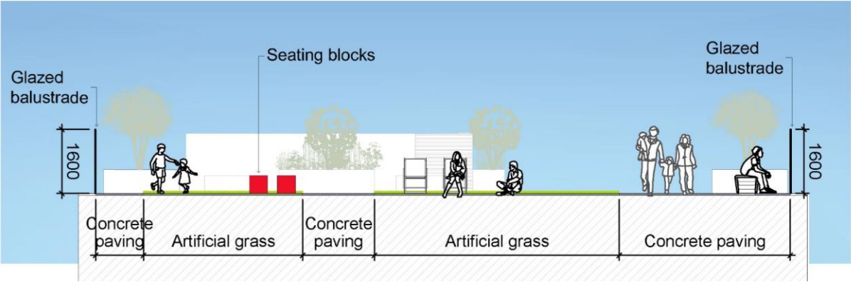
A - 12 th Floor Terrace Section
