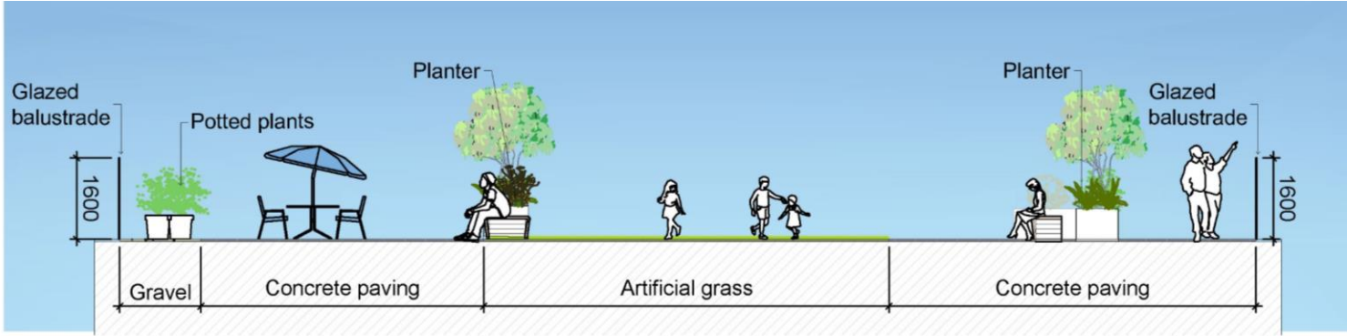
B - 9 th Floor Terrace Section
