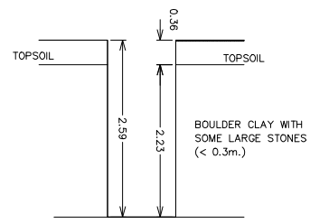
TRIAL HOLE NO. 1
