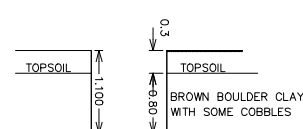
TRIAL HOLE NO. 22
