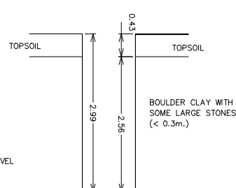
TRIAL HOLE NO. 8
