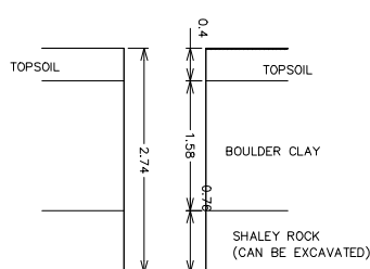
TRIAL HOLE NO. 2
