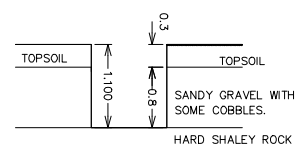
TRIAL HOLE NO. 16
