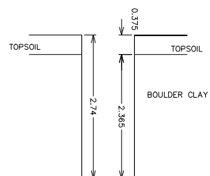
TRIAL HOLE NO. 12
