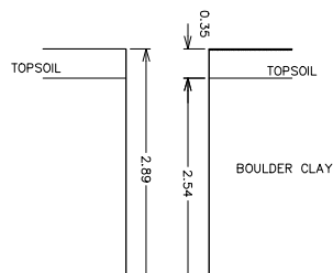
TRIAL HOLE NO. 3
