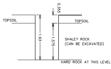
TRIAL HOLE NO. 6
