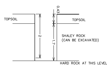
TRIAL HOLE NO. 5
