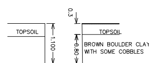
TRIAL HOLE NO. 19
