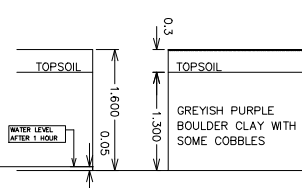
TRIAL HOLE NO. 26
