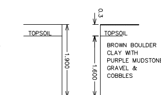
TRIAL HOLE NO. 21
