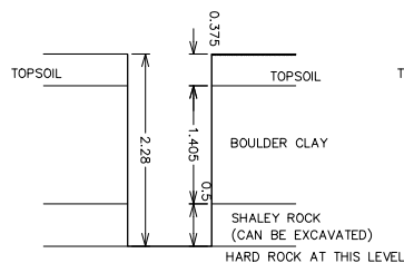
TRIAL HOLE NO. 7
