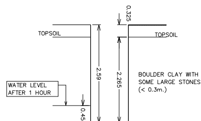
TRIAL HOLE NO. 15
