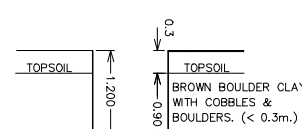
TRIAL HOLE NO. 23
