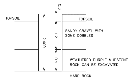
TRIAL HOLE NO. 18
