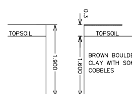
TRIAL HOLE NO. 25
