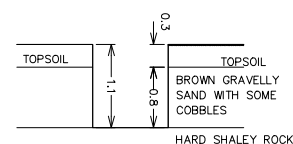
TRIAL HOLE NO. 17
