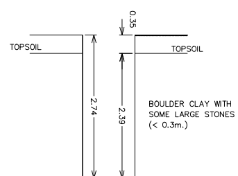
TRIAL HOLE NO. 9
