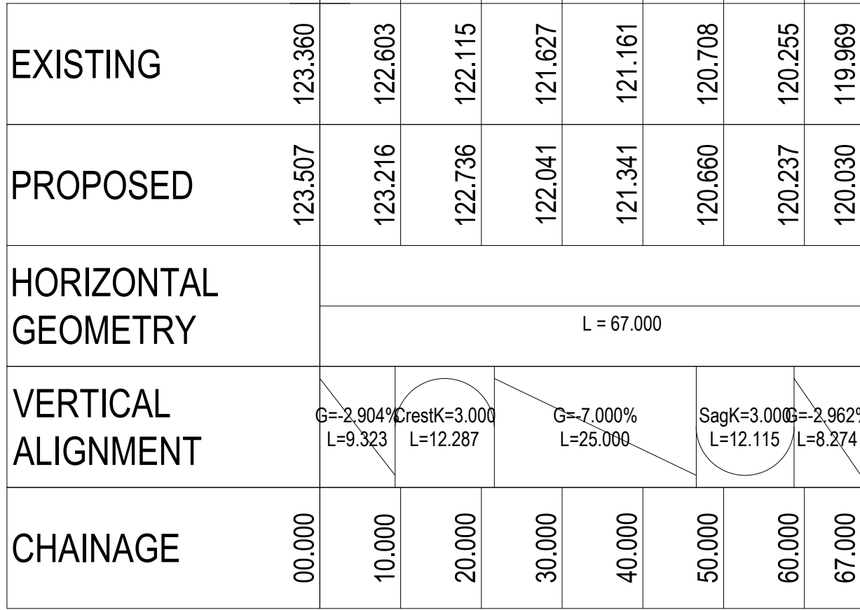
Title = SIDE ROAD 07 - LONGSECTION
