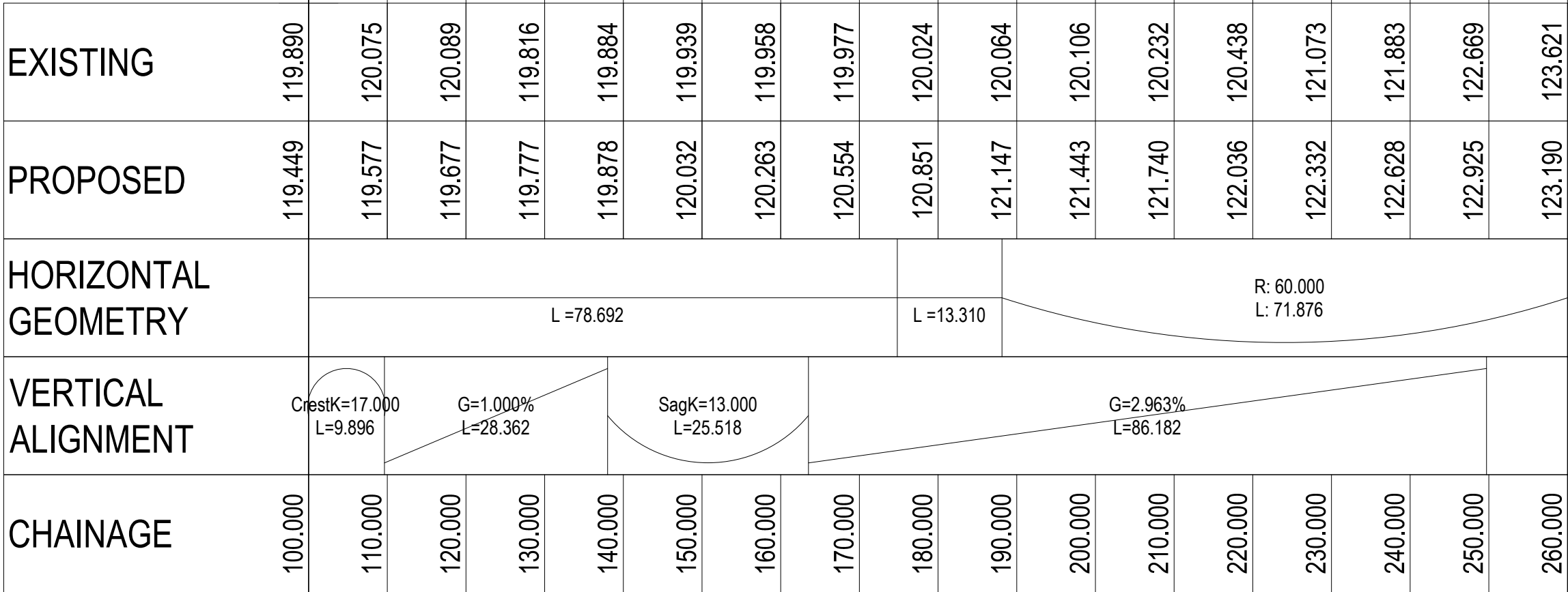
Title = MAIN ROAD 03 - LONGSECTION
