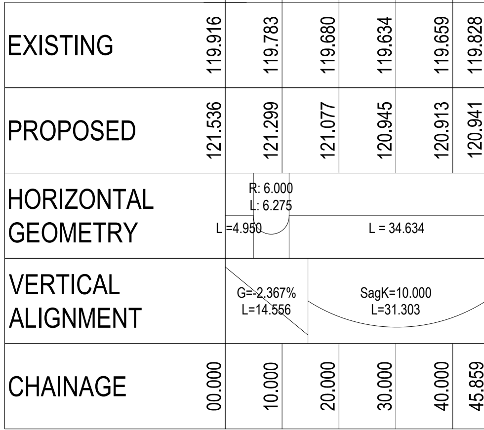
Title = SIDE ROAD 10 - LONGSECTION
