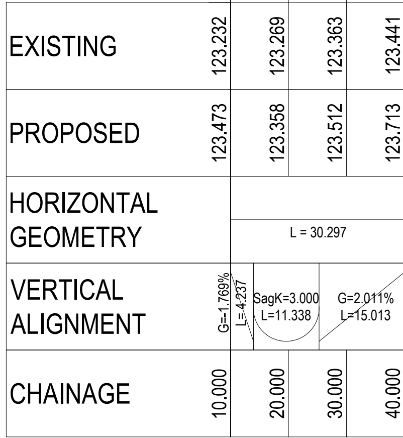
Title = SIDE ROAD 08 - LONGSECTION
