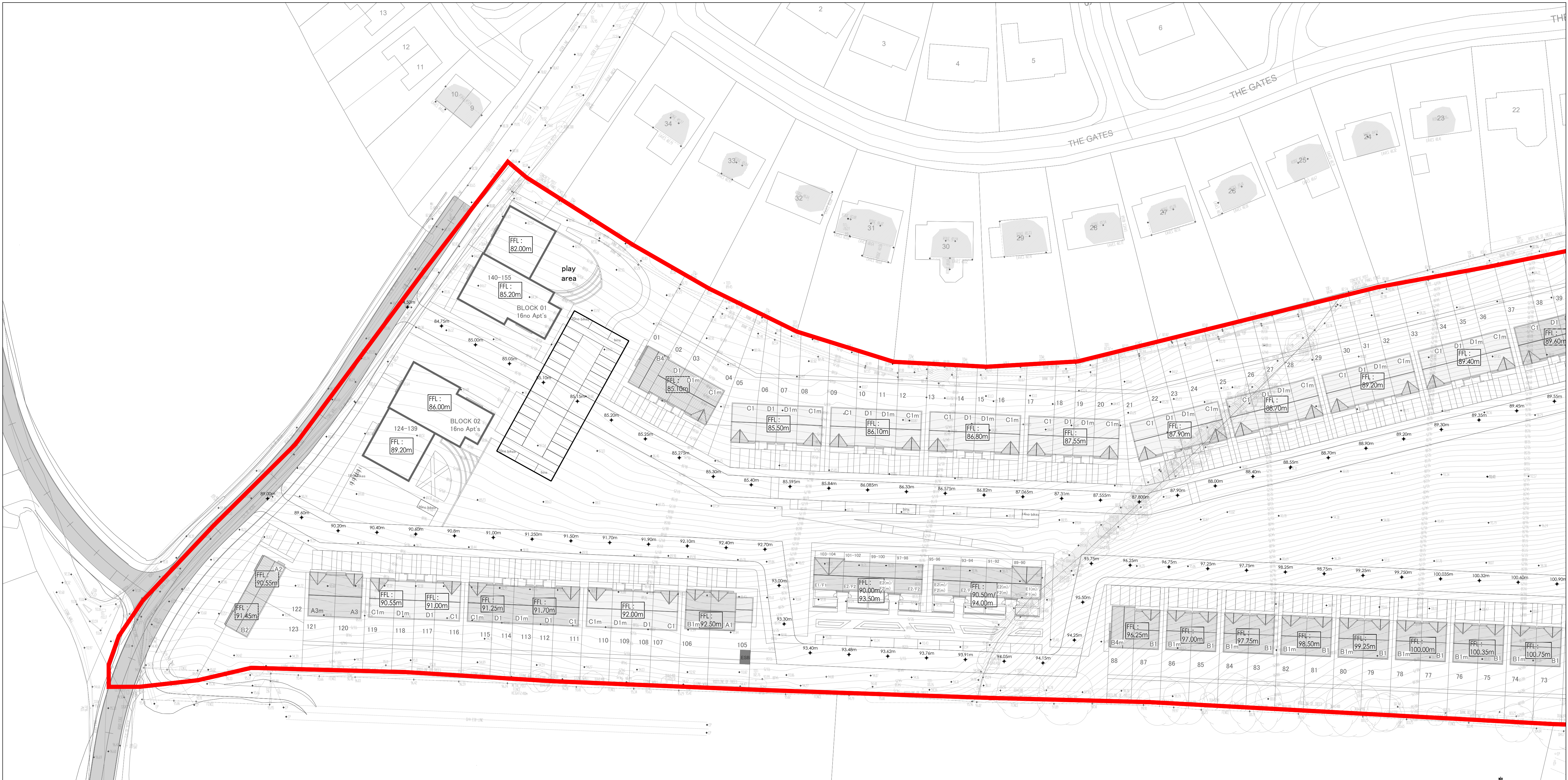
Proposed Internal Road & Levels Layout 1 of 2 Scale : 1:500
