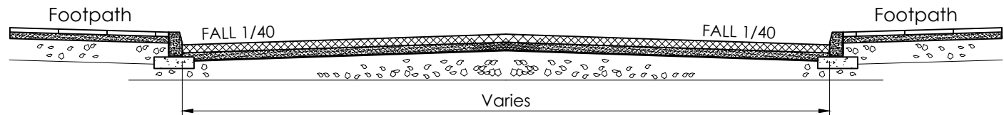
Typical Road Detail for Internal Estate Roads Scale 1:50
